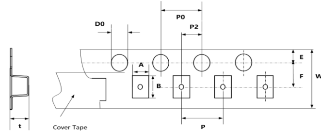
Fig. 5-6 0603,0805,1206,1210 (Plastic tape)
