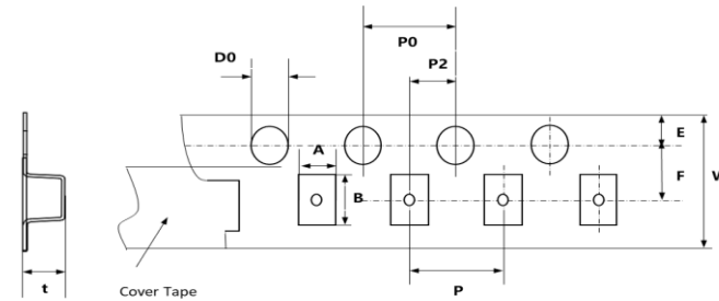
Fig. 7-5 0603,0805,1206,1210 ,2220 (Plastic tape)
