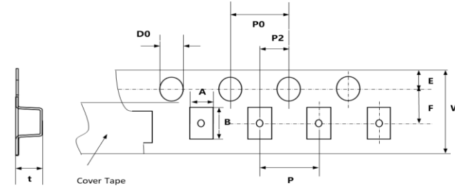
Fig. 5-6 0603,0805,1206,1210 (Plastic tape)
