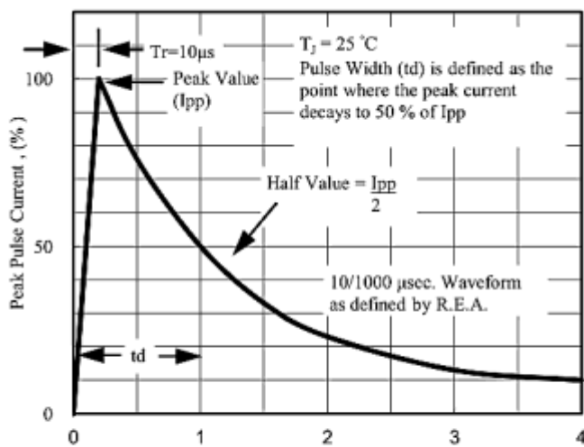
Fig. 5 - Pulse Waveform
